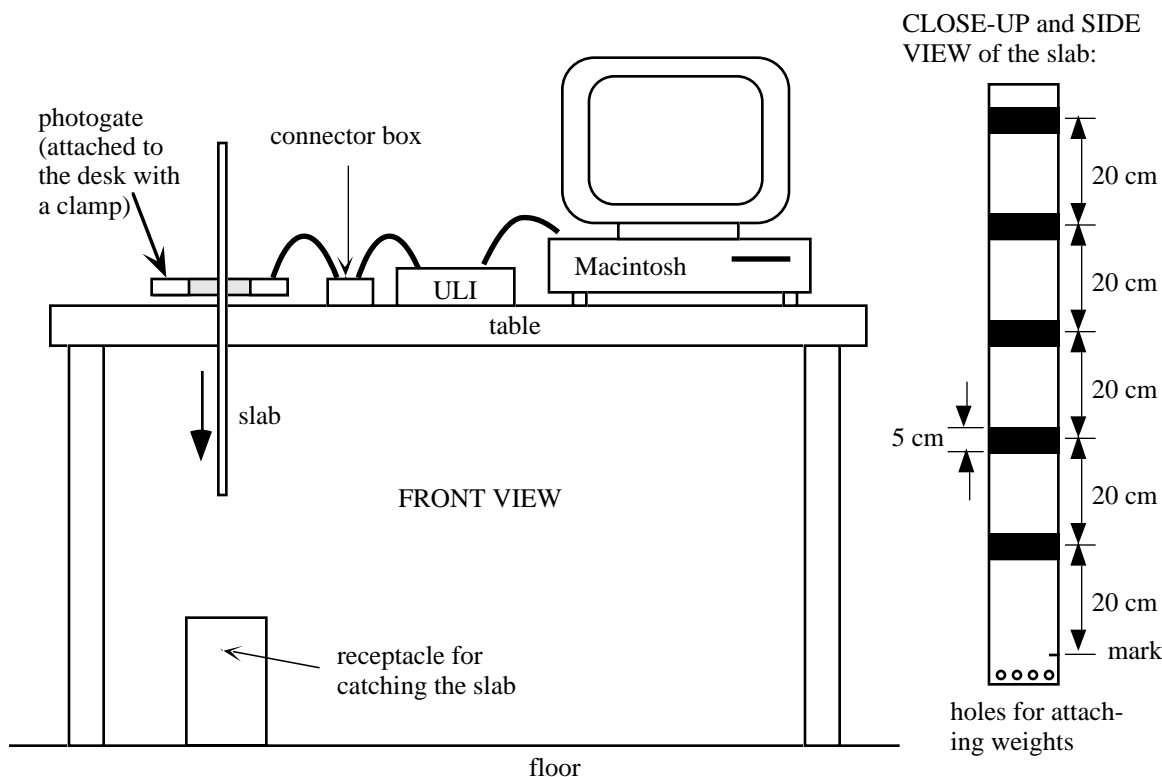
Figure 1: Sketch of the apparatus
